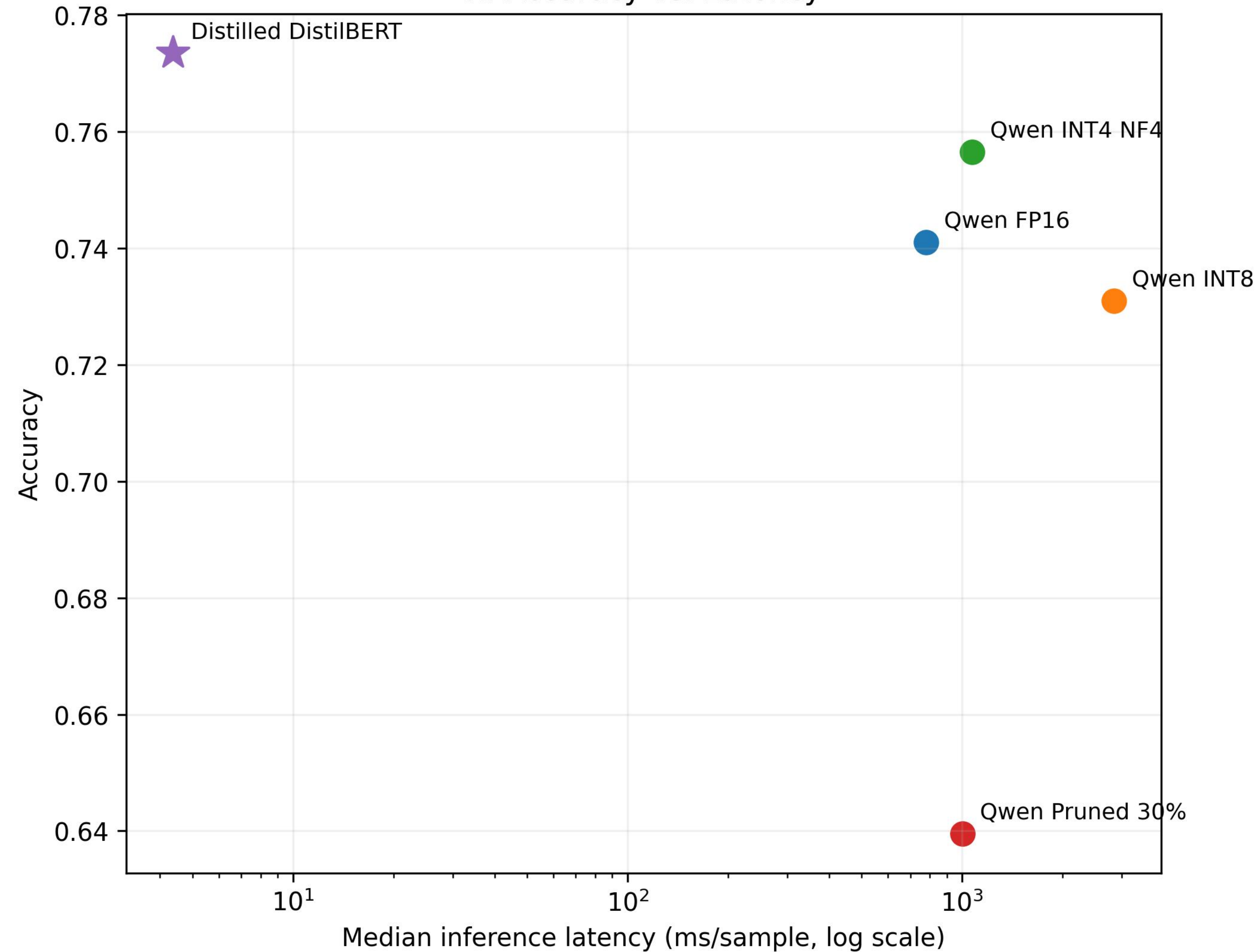
A. Accuracy vs. Latency
