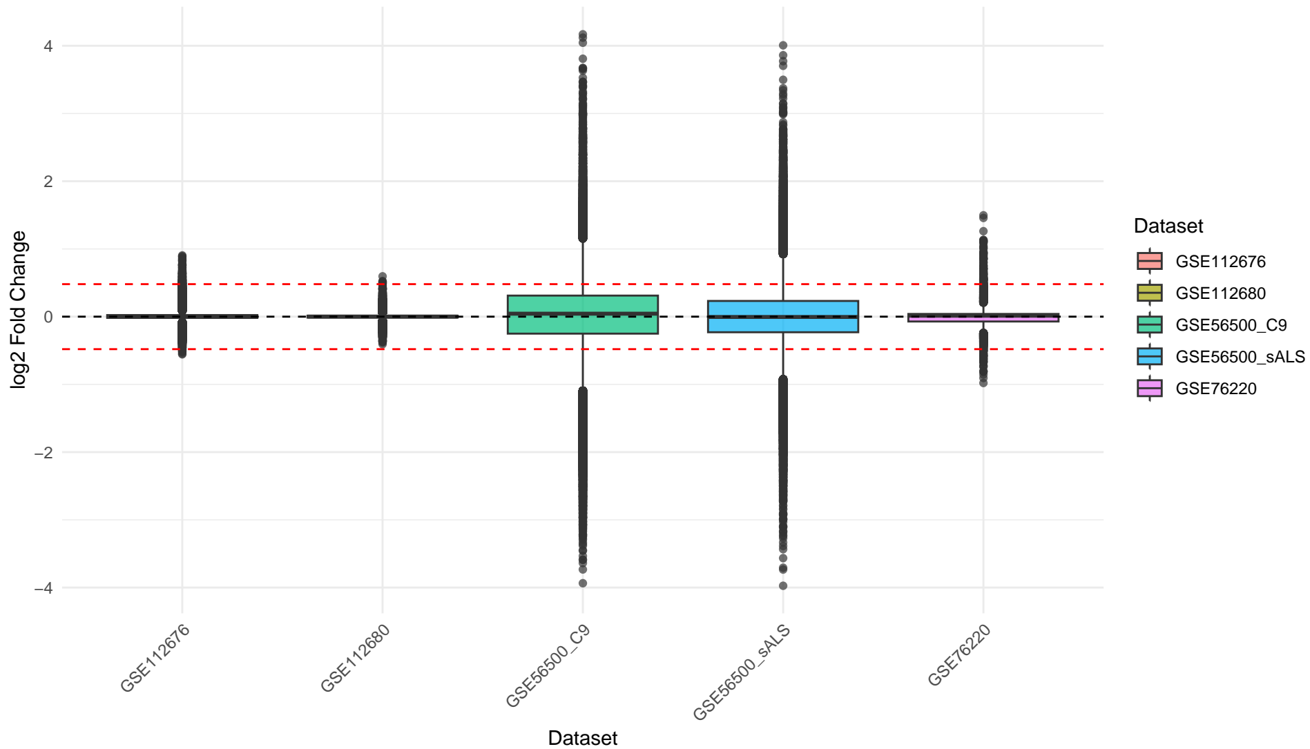
logFC Distributions – Boxplot
