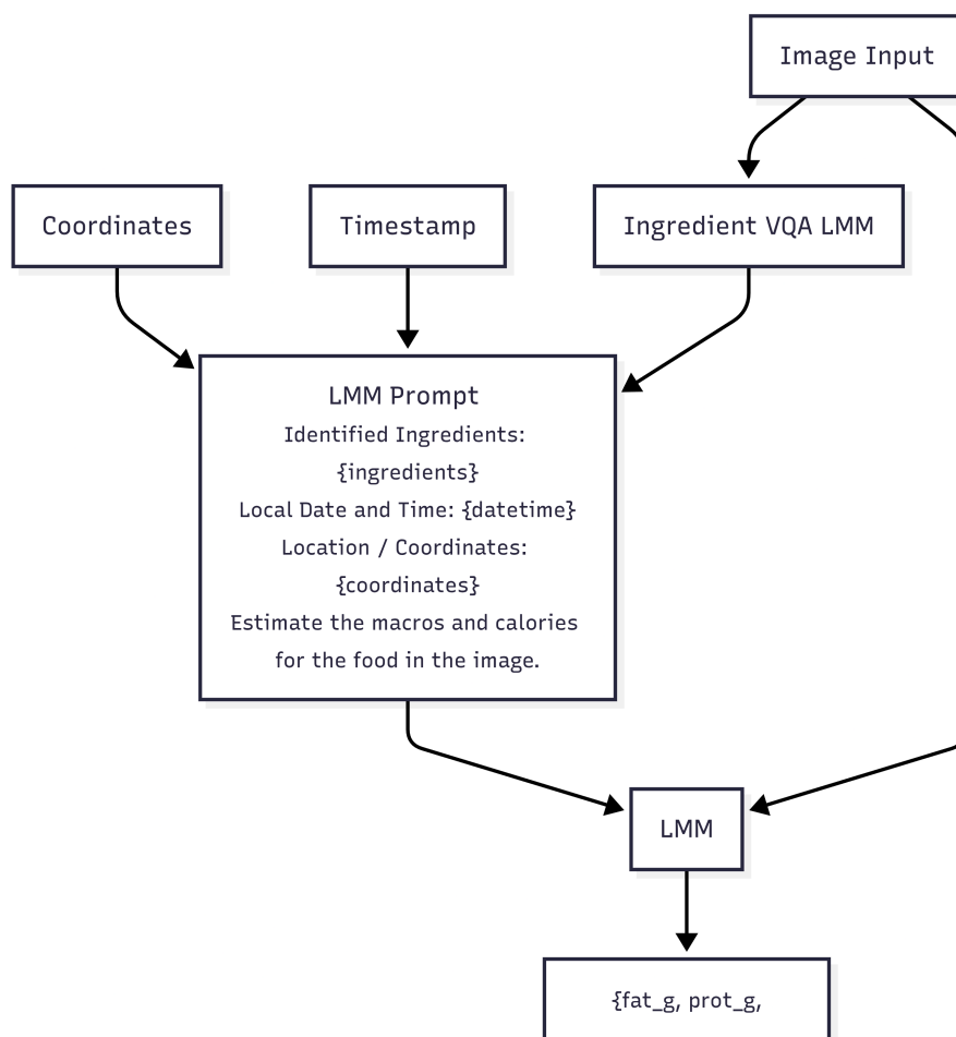
Figure 2: LMM enriched with metadata
