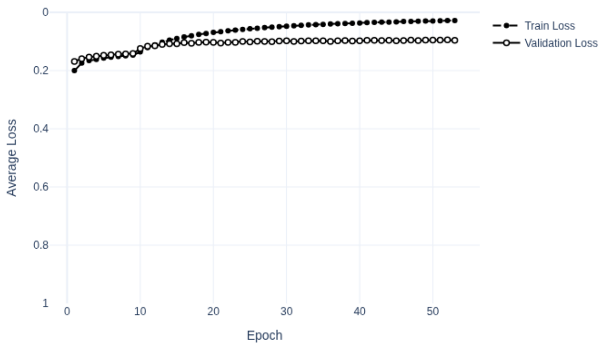
Loss vs Epochs for sequential_fine_tuning (Best Trial: 8)
