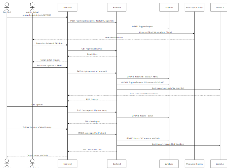
Gambar 3.15 Sequence Diagram 5: Helpdesk REVISION
