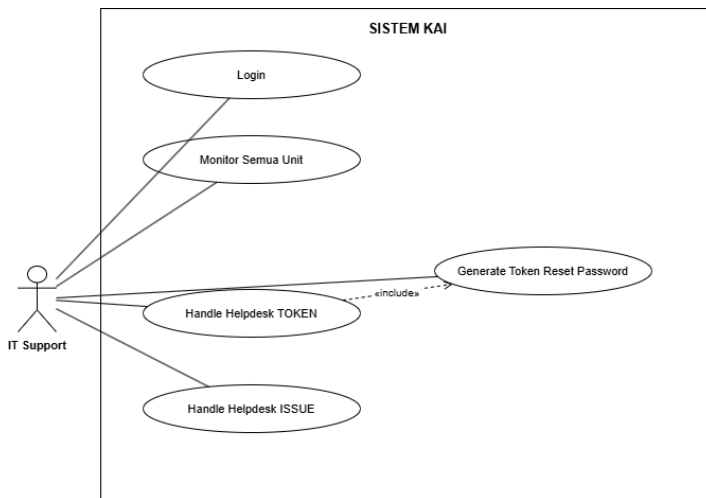
Gambar 3.4 Use Case Diagram Aktor IT Support
