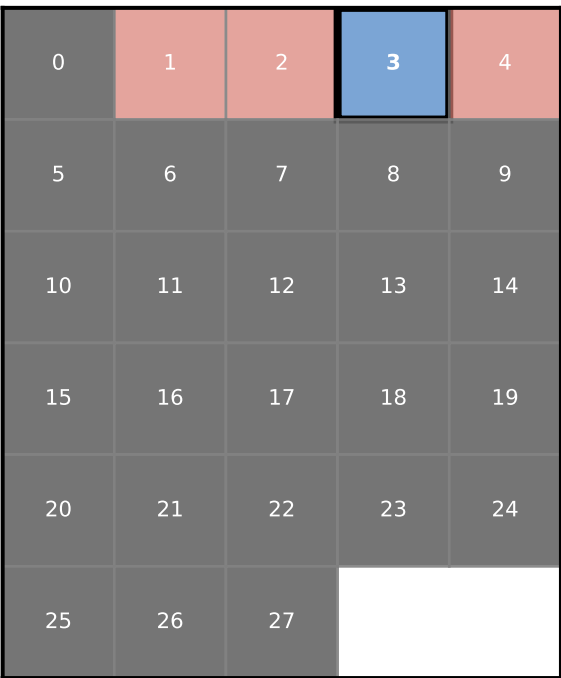
Qwen2.5-7B (Critical Layer: 3)
