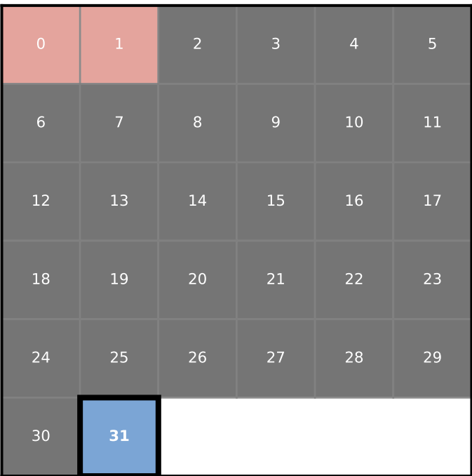
Mistral-7B (Critical Layer: 31)
