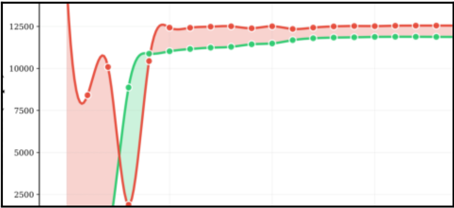
Qwen2.5-7B
