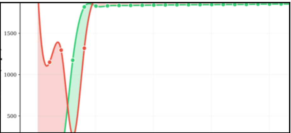
Falcon-7B
