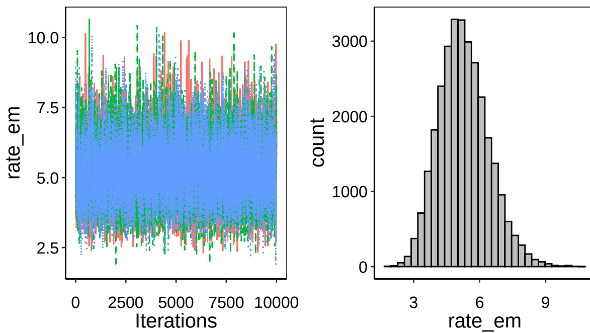
Figure 3: Convergence figures for gamma parameters for existing source MACT floor analysis for chemical X in subcategory A.
