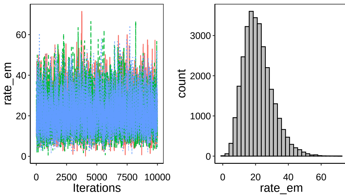
Figure 6: Convergence figures for skew-normal parameters for new source MACT floor analysis for chemical X in subcategory A.
