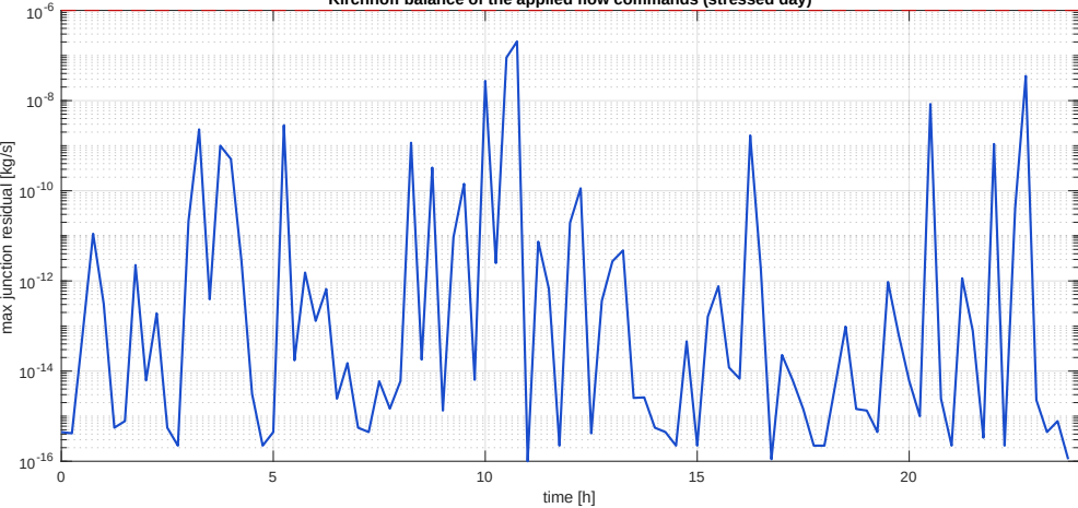
Kirchhoff balance of the applied flow commands (stressed day)
