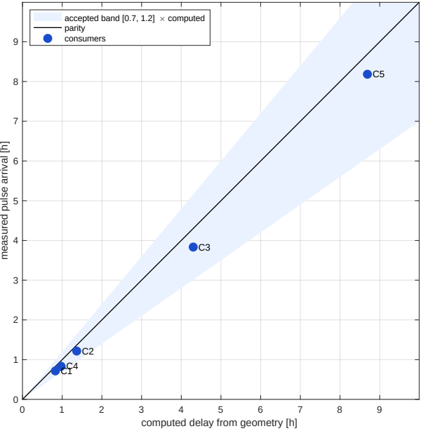
Transport delay: measurement vs geometry
