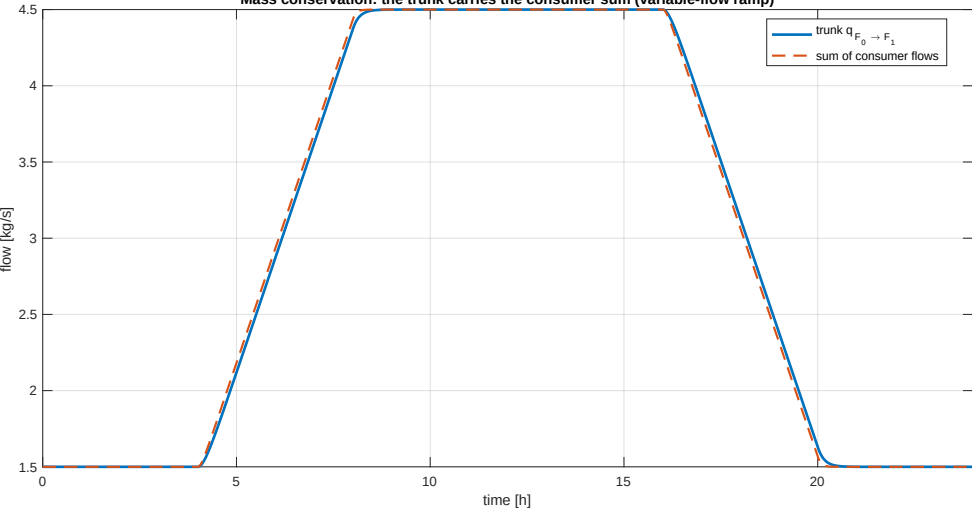
Mass conservation: the trunk carries the consumer sum (variable-flow ramp)
