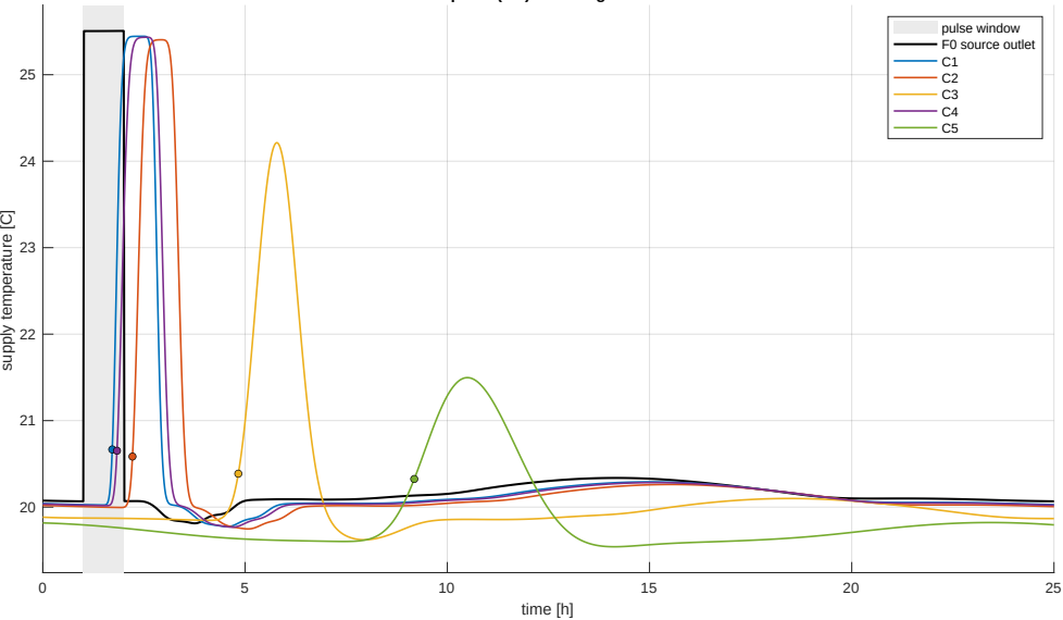
+5 K source pulse (1 h) travelling to the consumers
