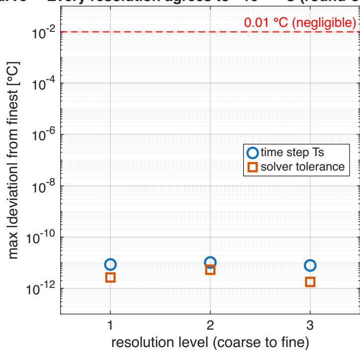
Every resolution agrees to \sim 10^{-11} °C (round-off)
