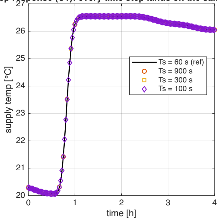
Step response (C1): every time step lands on the same curve
