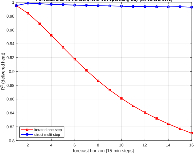
Forecast skill vs horizon, held-out operating day (all consumers)
