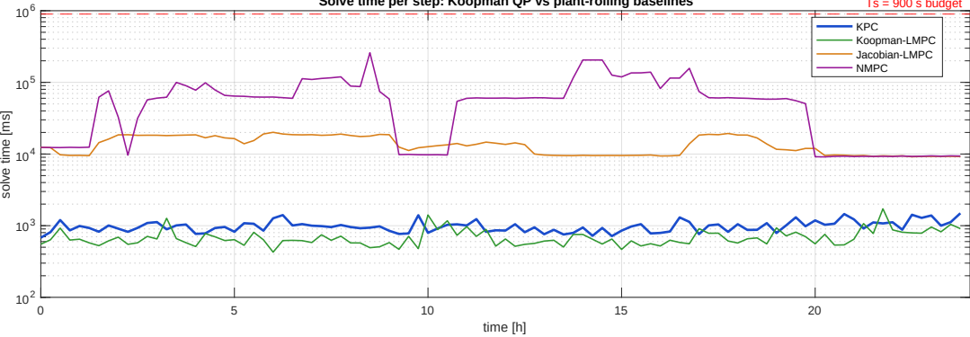
Solve time per step: Koopman QP vs plant-rolling baselines
