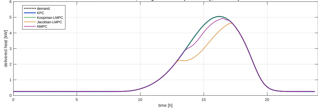
Delivered vs demand, binding consumer C3 (stressed day, \dot{m} = 0.35 )
