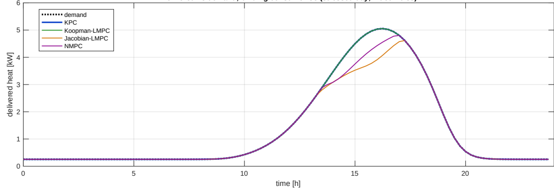
Delivered vs demand, binding consumer C3 (stressed day, \dot{m}_{\text{dot}} = 0.35 )
