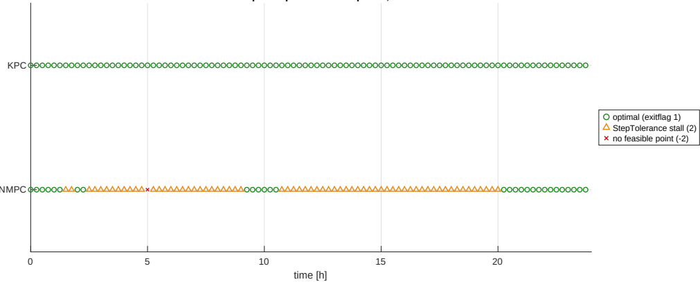
Solver certificate per step: KPC 96/96 optimal, NMPC 29/96
