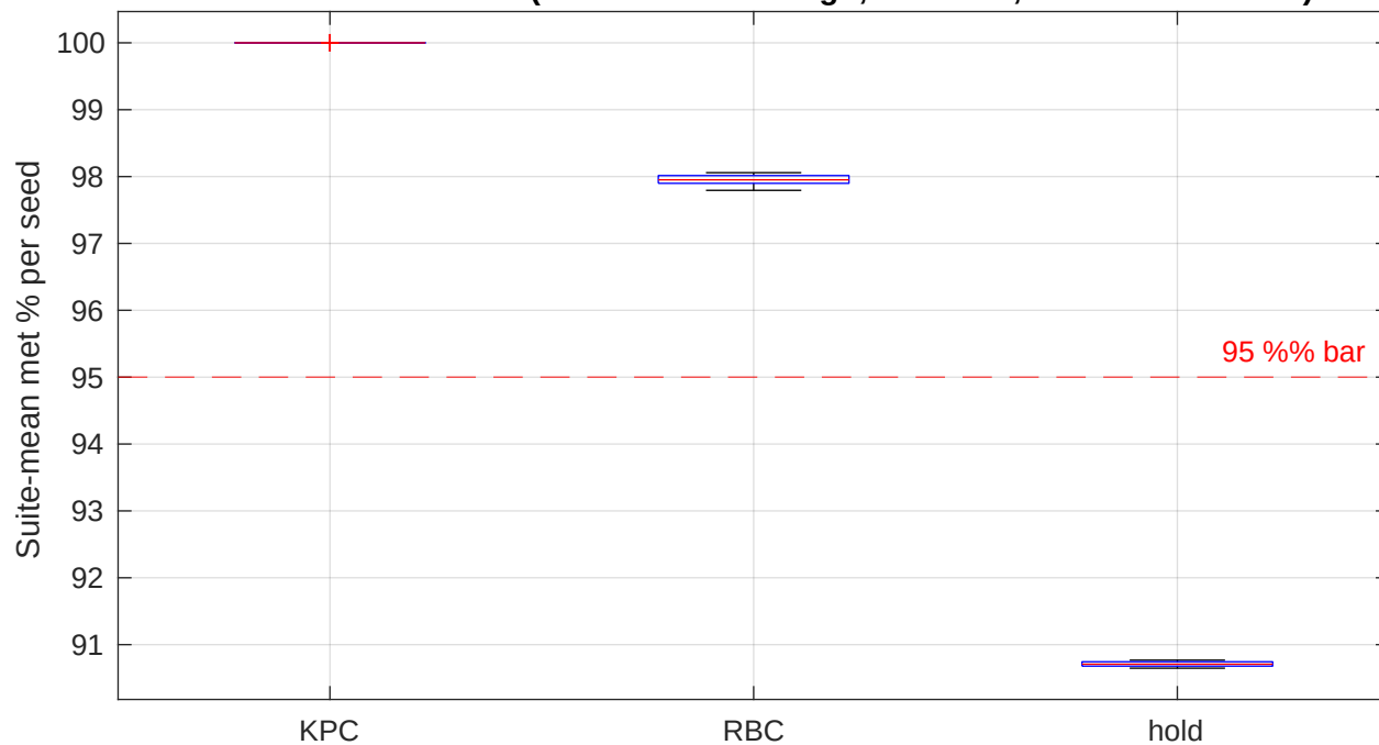
Stressed Monte Carlo (mdot = 0.60 x design, 30 seeds, Cohen's d = 31.81)
