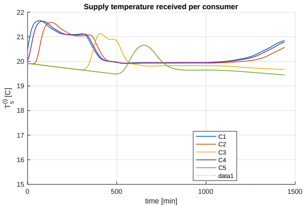
variable flow | time-varying flow 0.5x to 1.5x ramp, T_0s = 20 , 12:30 start (dynamic-flow check)
