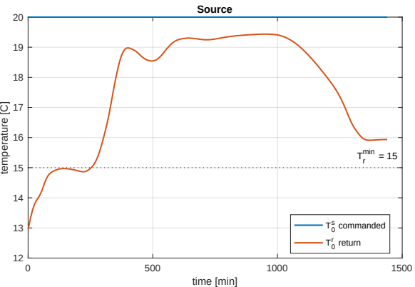
variable flow | time-varying flow 0.5x to 1.5x ramp, T_0s = 20 , 12:30 start (dynamic-flow check)
