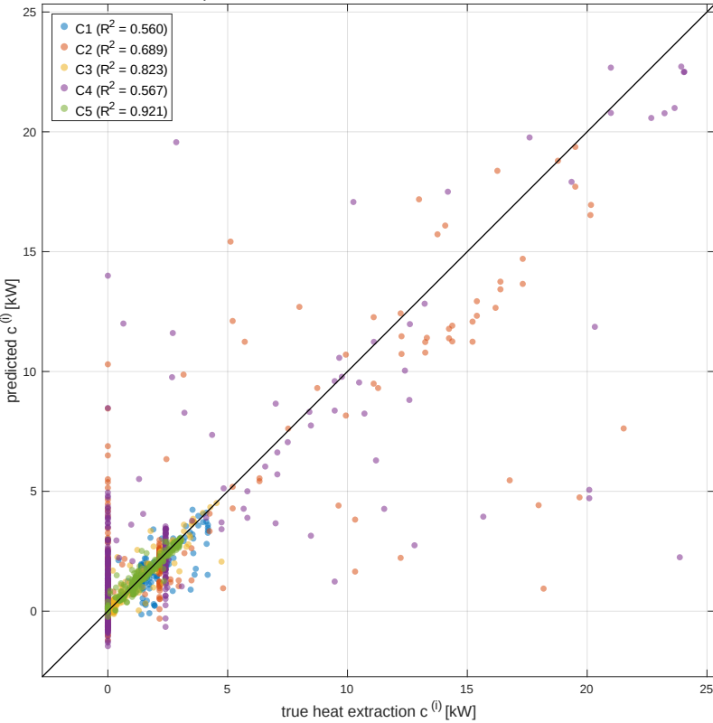
V_{seq} 1-step prediction on test trajectories, suite R^2 = 0.712
