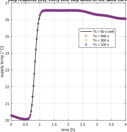
Step response (C1): every time step lands on the same curve
