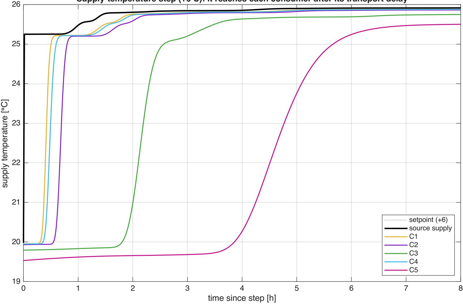
Supply-temperature step (+6 C): it reaches each consumer after its transport delay
