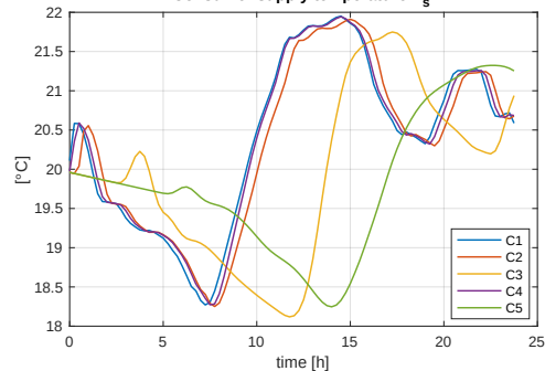
Consumer supply temperature T_s^{(i)}
