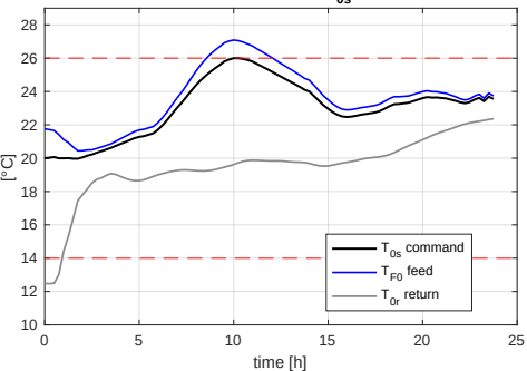
Source temperatures (command T_{0s} bounded 14-26 C)
