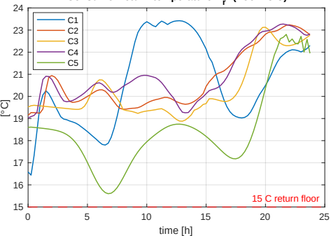
Consumer return temperature T_r^{(i)} (floor 15 C)
