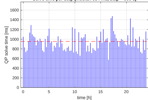
Solve time per step (median 954 ms, step = 900 s)
