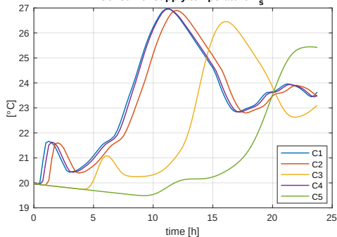
Consumer supply temperature T_s^{(i)}
