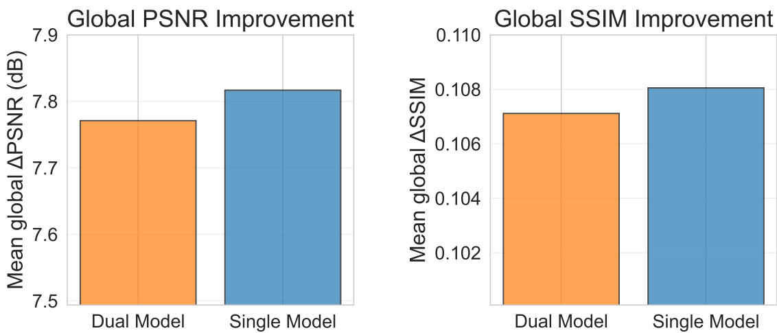
Fig.5.17 Global PSNR and SSIM improvement over the corrupted input for the Single and Dual Models on the test set.
