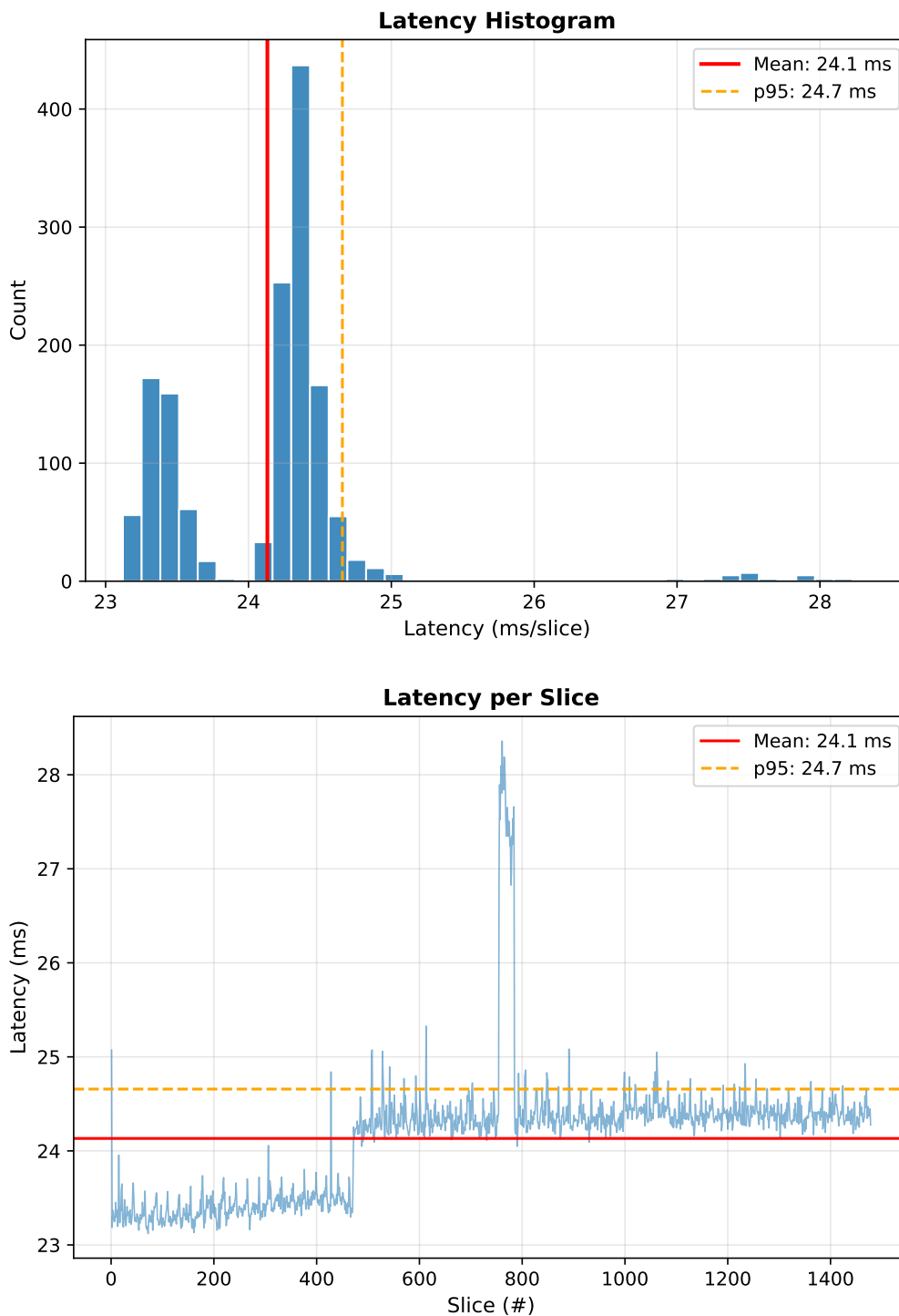
Fig.5.18 Inference benchmark: latency histogram and latency per slice.
