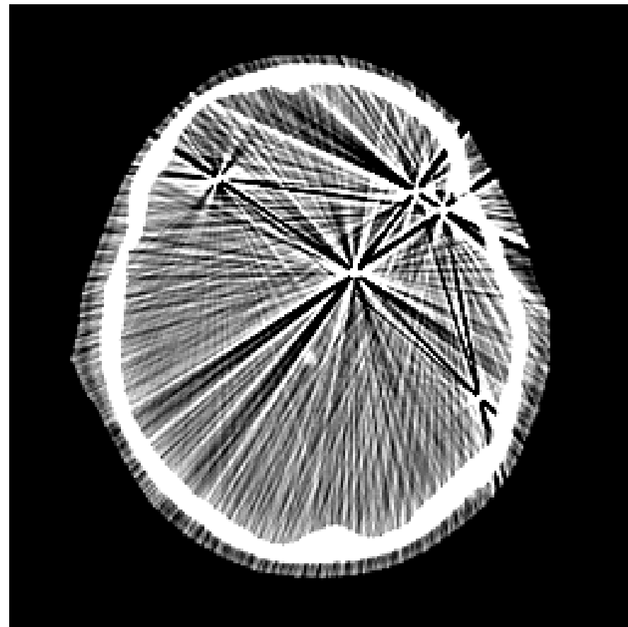
Artifact-Affected Input
