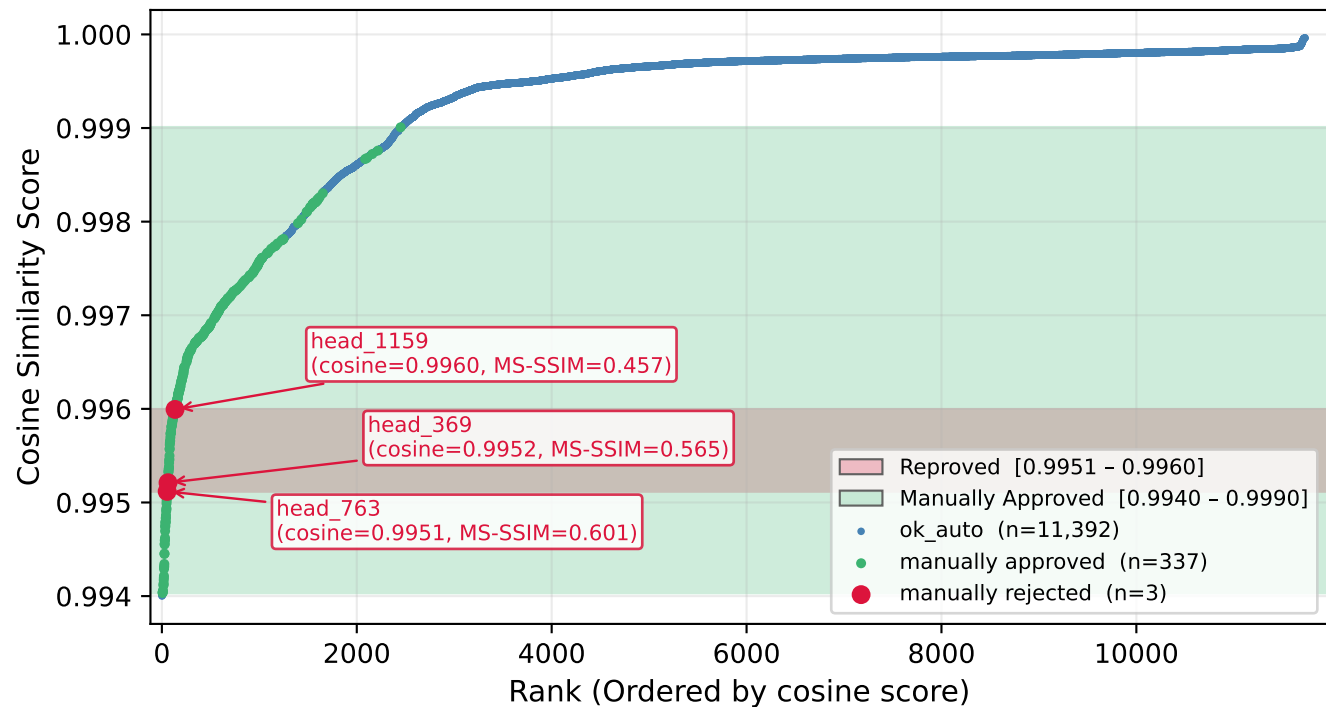
Cosine Similarity — Same 11,732 pairs audited with MS-SSIM
