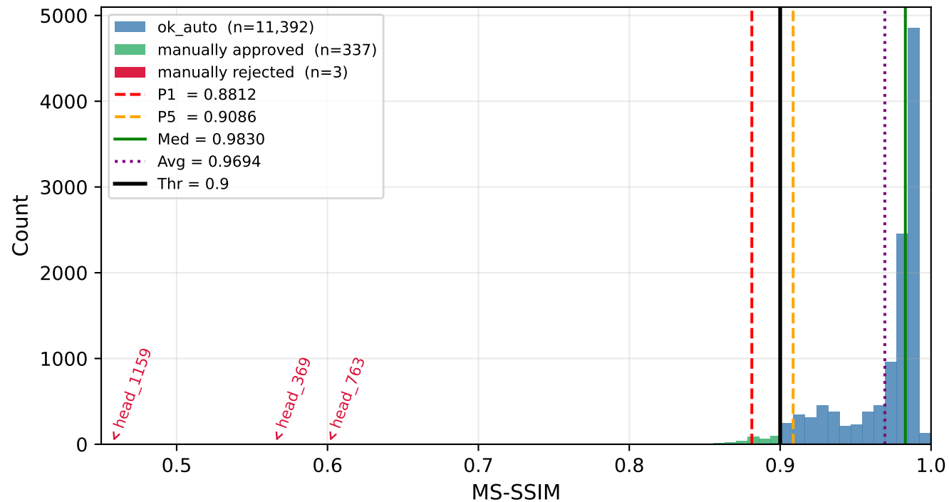
MS-SSIM distribution — (n=11,732) (clean CTMAR vs DL/Stroke)
