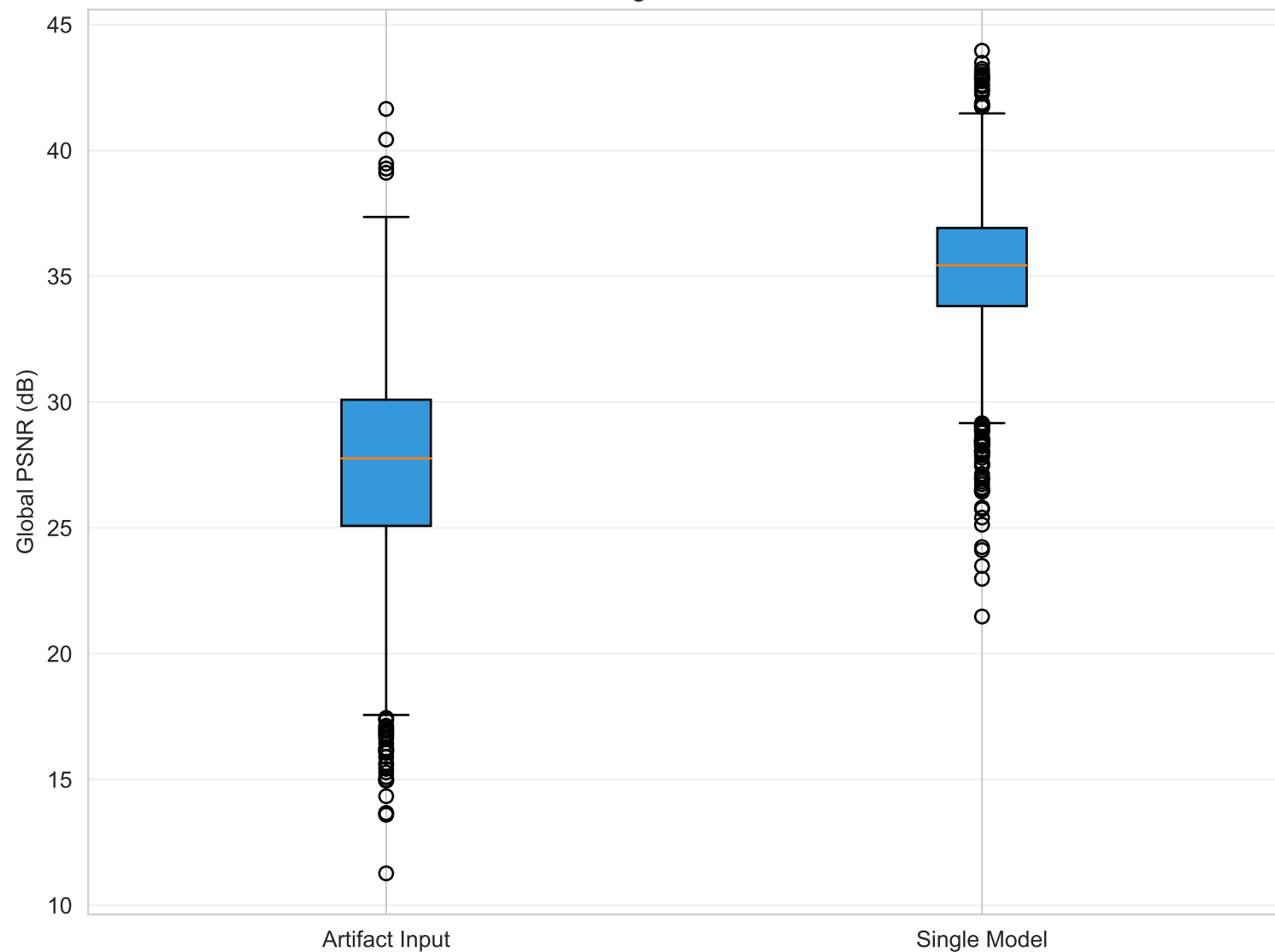
Per Image Global PSNR
