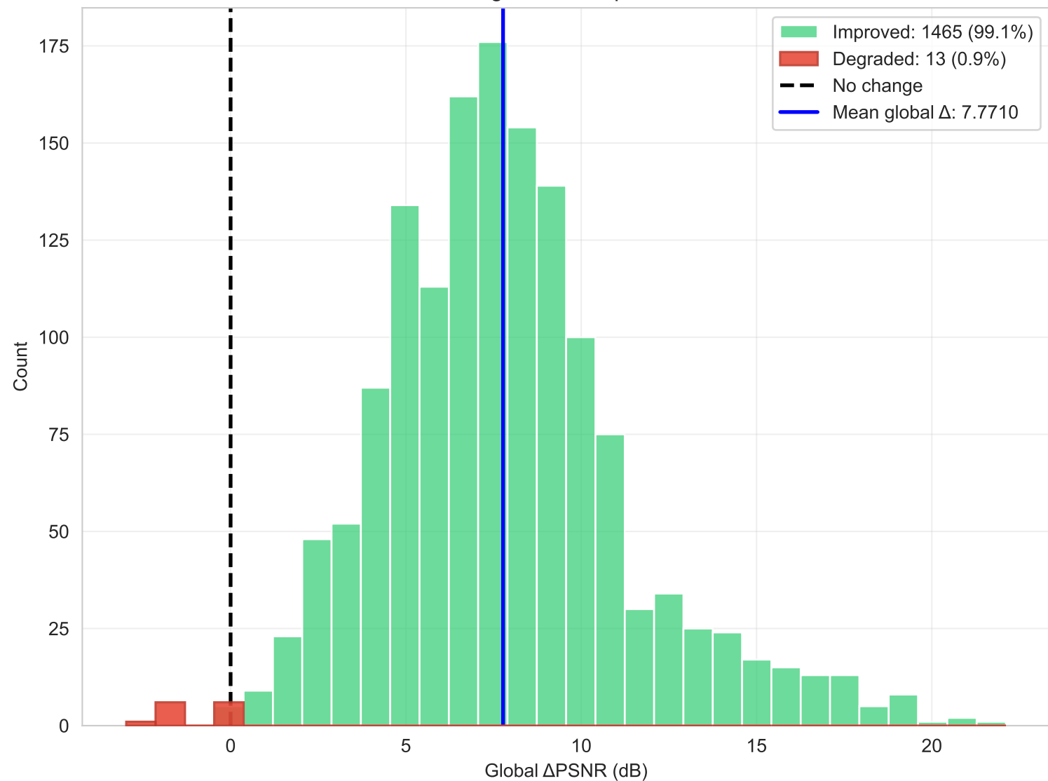
Per Image PSNR improvement
