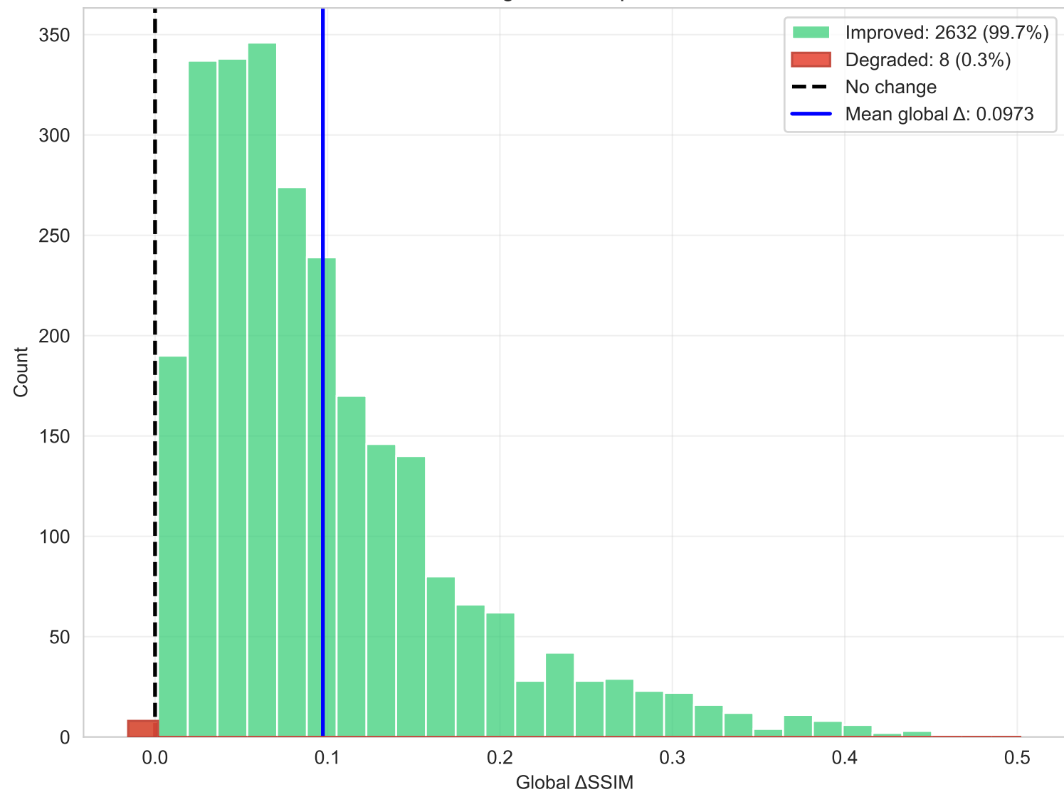
Per Image SSIM improvement
