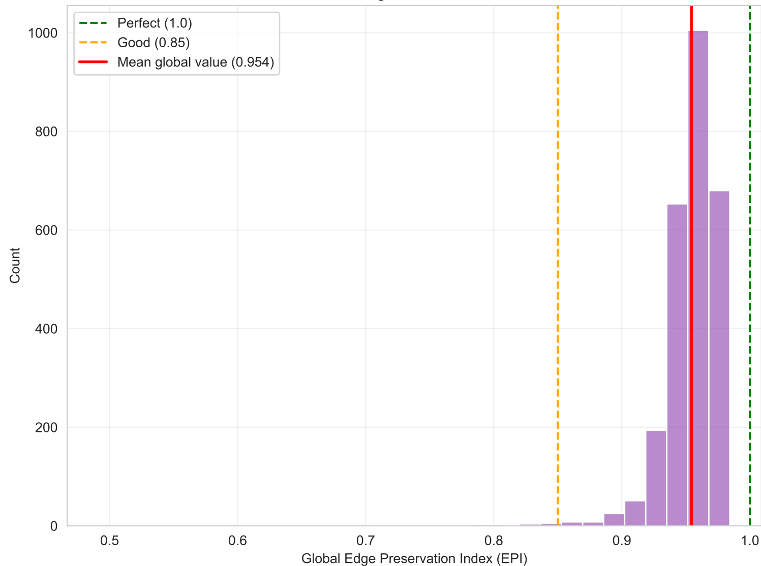
Per Image EPI distribution
