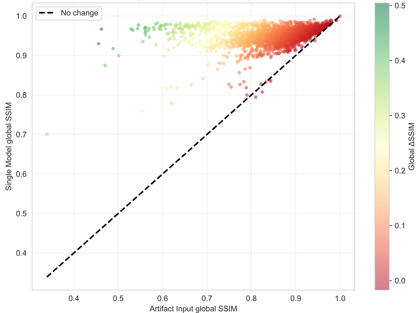
Global SSIM: Artifact Input vs Model (Above line = improvement)
