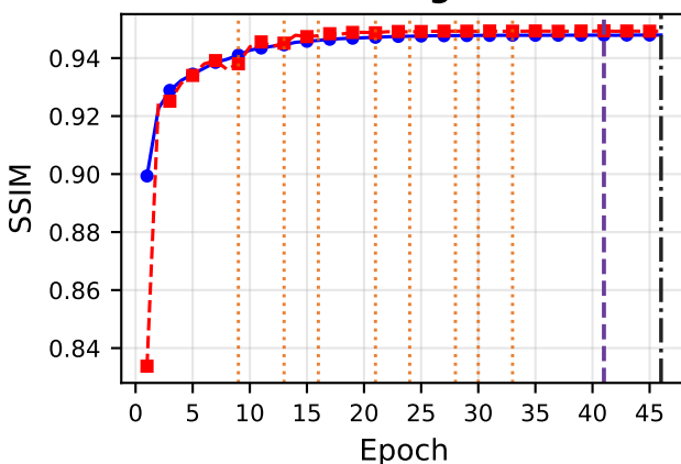
Global Image SSIM
