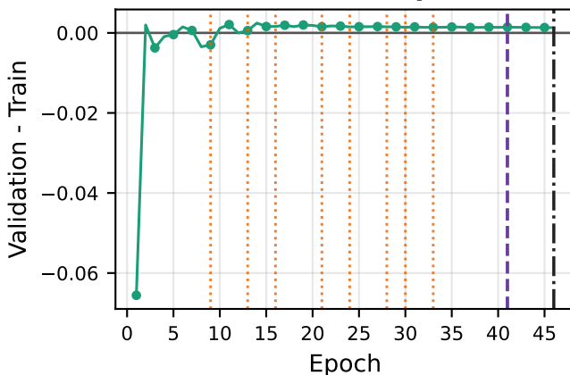
Generalization Gap (SSIM)
