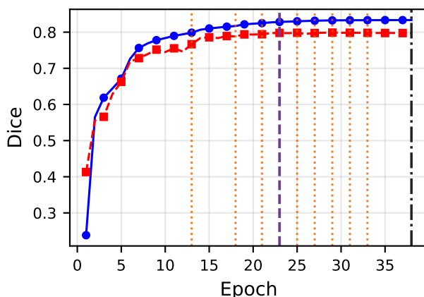
Artifact Mask Dice Score
