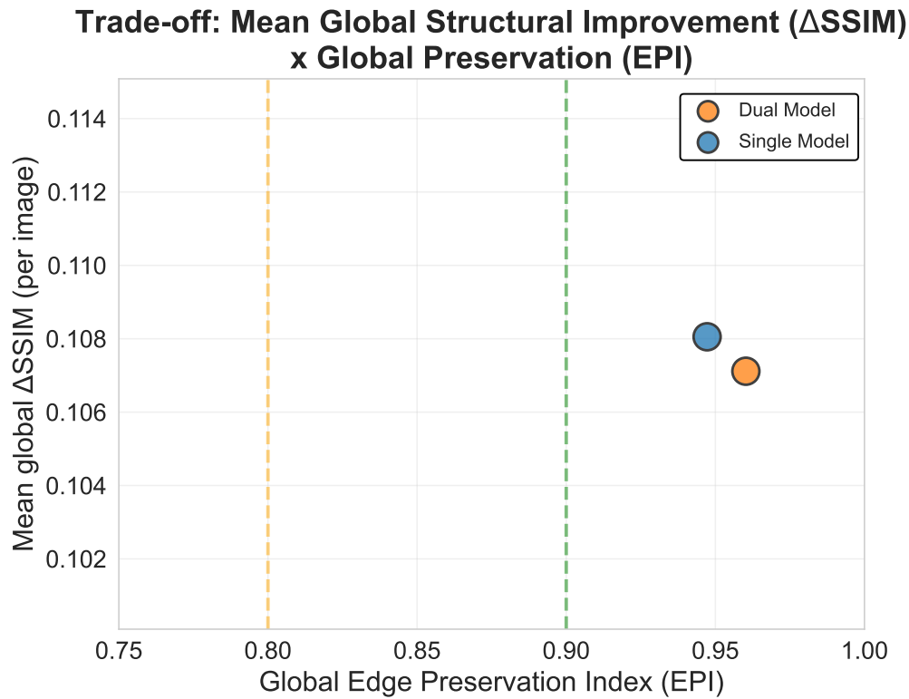
Fig.5.18 Global trade-offs between mean structural improvement ( \Delta SSIM) and preservation: texture preservation score (top) and edge preservation index (bottom), for the Single and Dual Models selected with seed 2024 on the test set.
