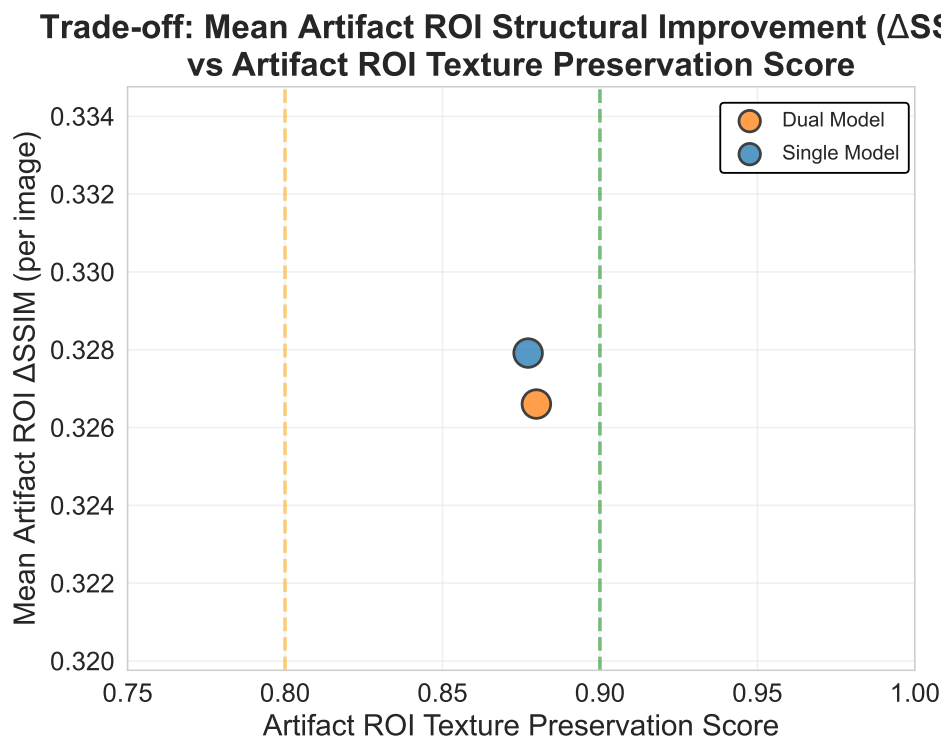
Fig.5.19 Artifact ROI trade-offs between mean structural improvement ( \Delta SSIM) and preservation: edge preservation index (top) and texture preservation score (bottom), for the Single and Dual Models selected with seed 2024 on the test set.
