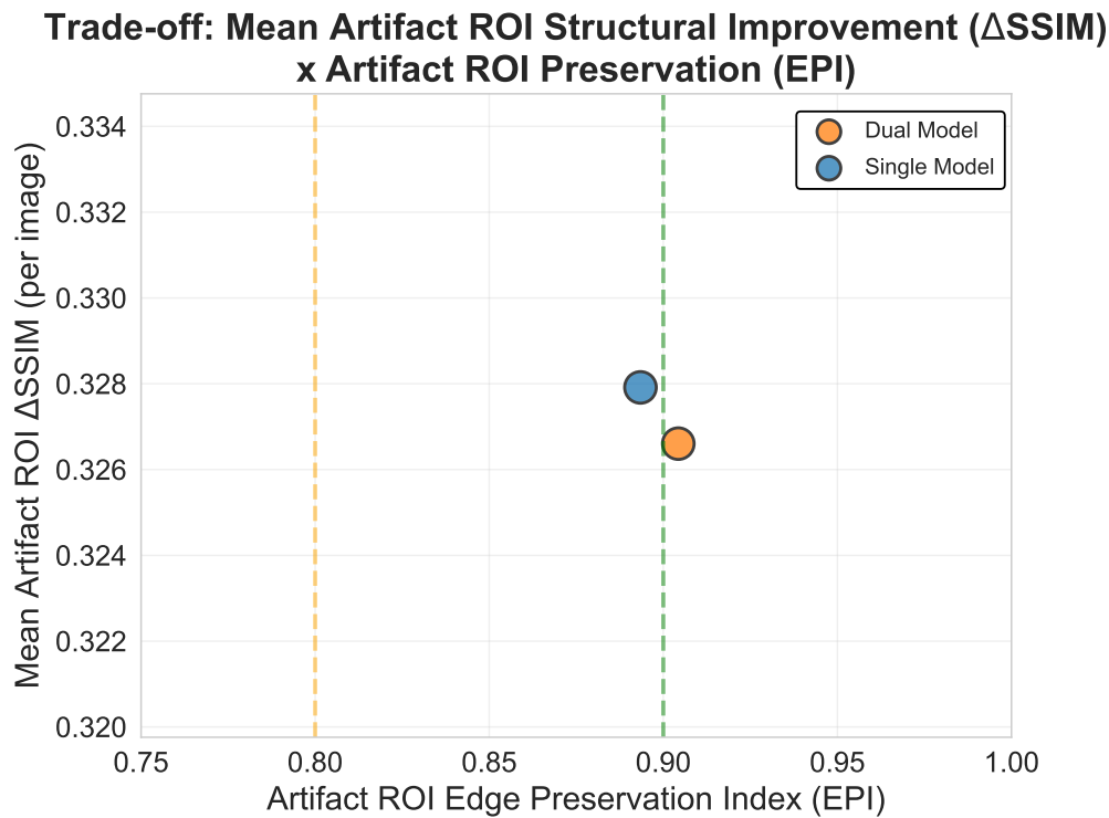
Fig.5.18 Global trade-offs between mean structural improvement ( \Delta SSIM) and preservation: texture preservation score (top) and edge preservation index (bottom), for the Single and Dual Models selected with seed 2024 on the test set.
