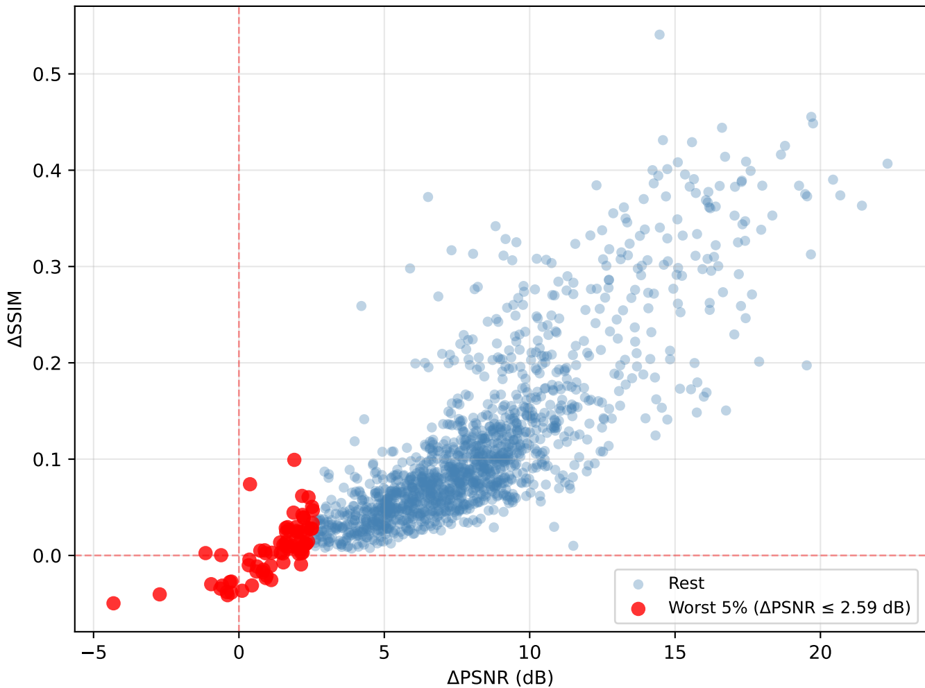
Worst-Case Samples (N=74 Highlighted in Red)
