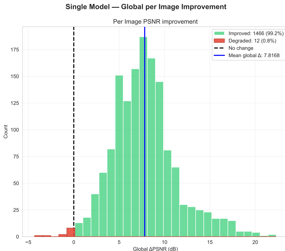
Fig.5.11 Per-image global improvement over the corrupted input for the Single Model, seed 2024: \Delta SSIM (top) and \Delta PSNR (bottom). Green bars indicate improvement and red bars indicate degradation. The distributions are descriptive; inferential analyses used patient-level aggregation.
