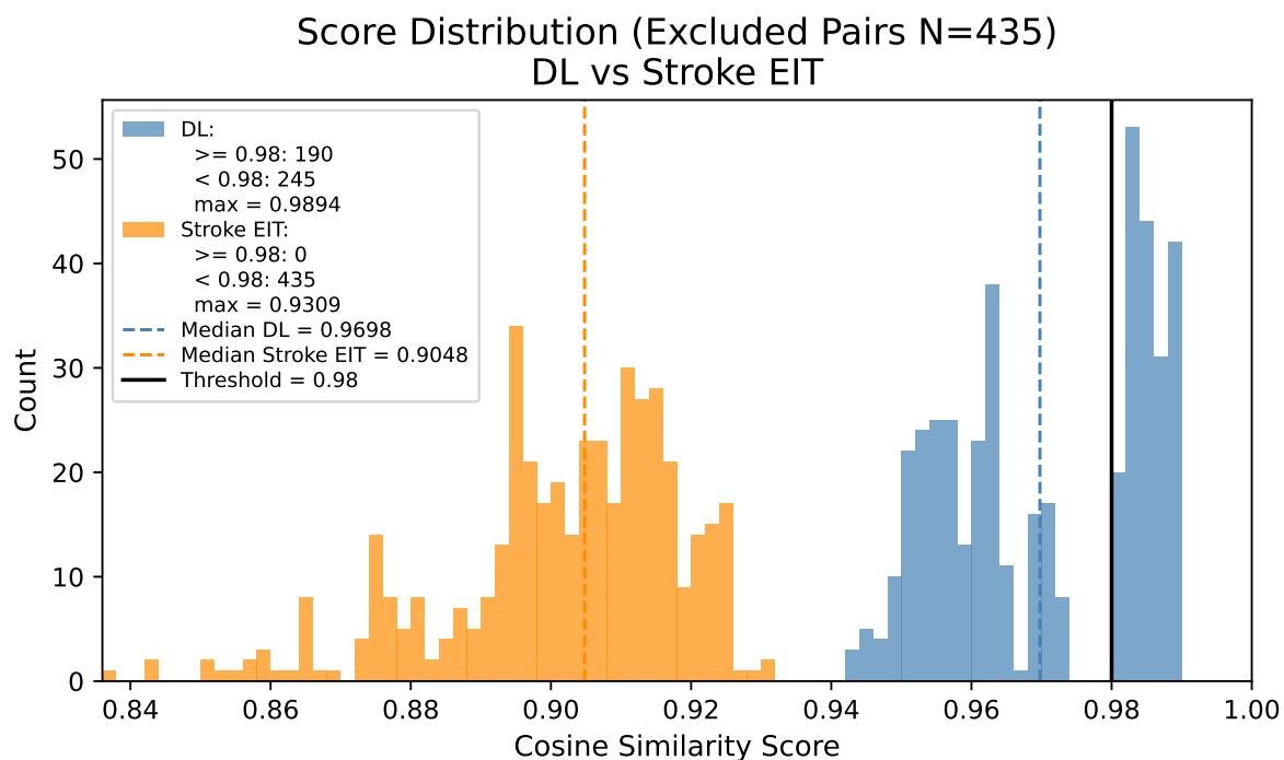
Fig.5.8 Score distribution of excluded pairs (DL x Stroke EIT) for pairs without approved matches in either of the two source datasets (N=435). The orange histogram shows the distribution of scores for the 435 pairs rejected in the Stroke EIT Dataset. The blue histogram shows the distribution of the same 435 pairs rejected in the Deep Lesion Dataset.
