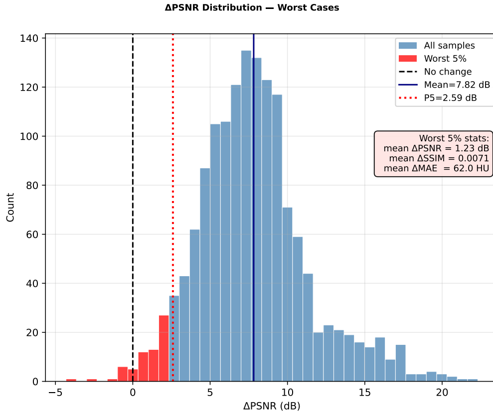
Fig.A.11 Bottom 5th-percentile slices by global \Delta\text{PSNR} for the Single Model, seed 2024, test split ( N = 74/1478 , threshold = 2.59 dB, highlighted in red). Descriptive. No inferential test is derived from this subset.
