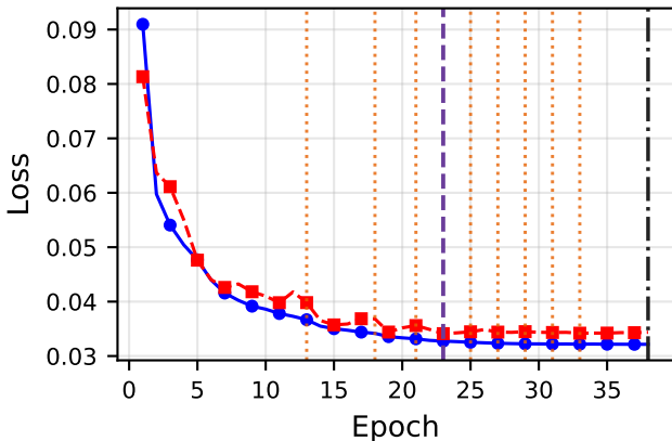
Loss Total
