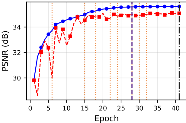
Global Image PSNR
