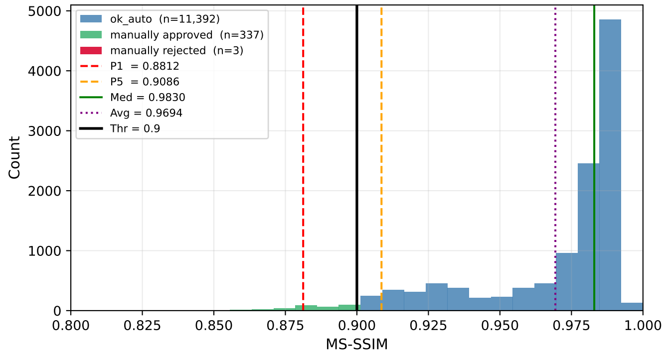
MS-SSIM distribution — Zoom (clean CTMAR vs DL/Stroke)
