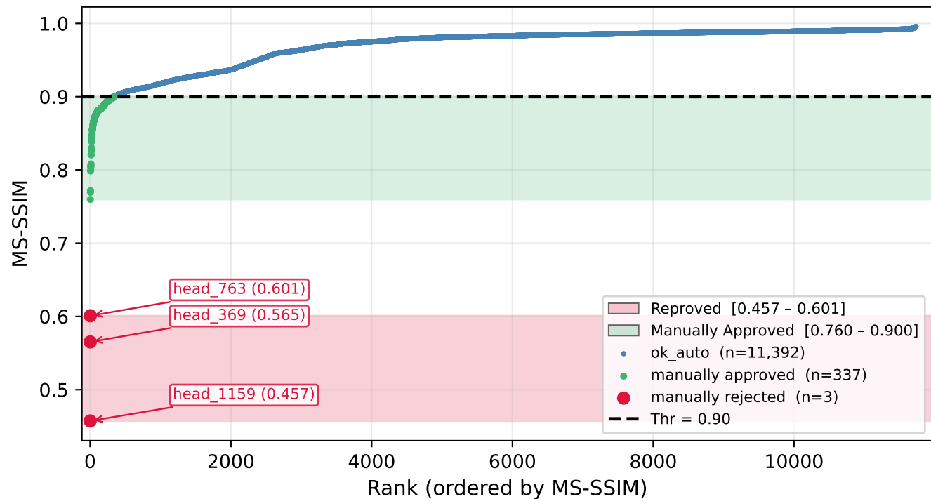
MS-SSIM distribution (clean CTMAR vs DL/Stroke; N=11,732)
