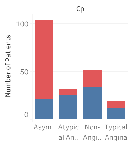
Chest Pain (CP) type per target
