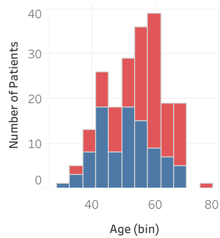
Age distribution per target
