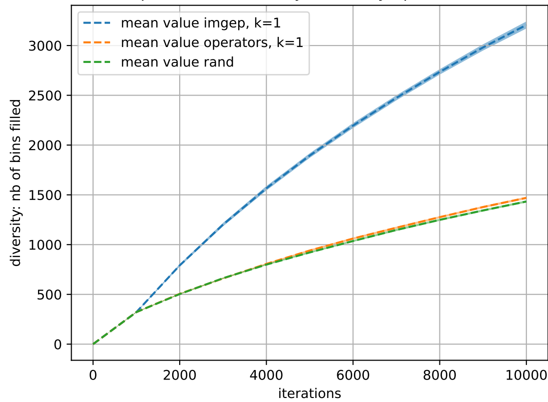
Miss and hit subspace mean diversity, 95 % asymptotic CI interval, 500 run
