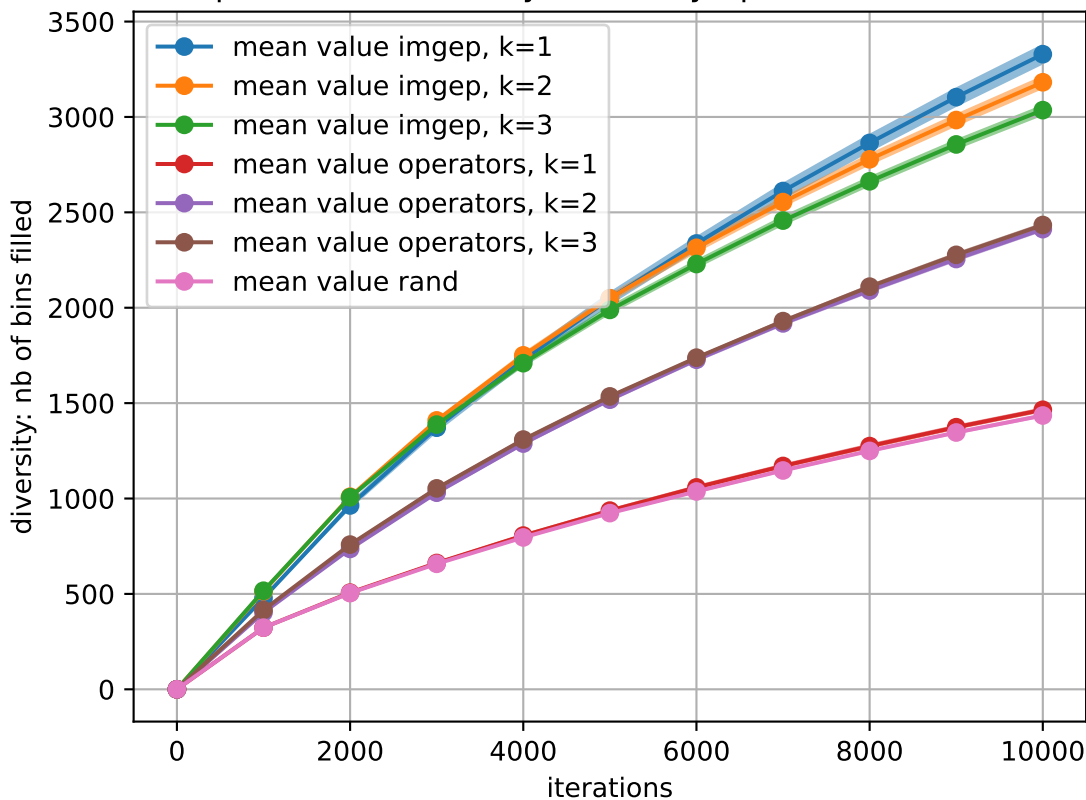
Time subspace mean diversity, 95 % asymptotic CI interval, 500 runs
