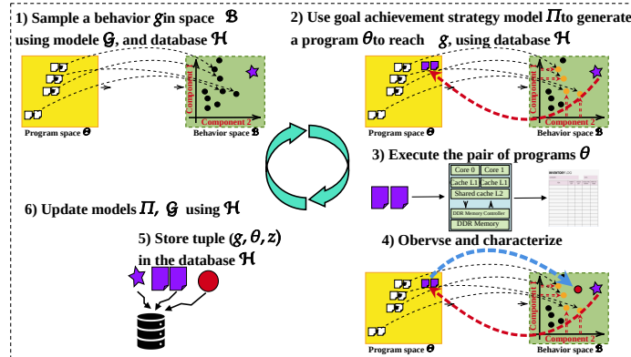
Figure – Schematic view of an IMGEP for our case of interference identification, based on the general description of IMGEP
