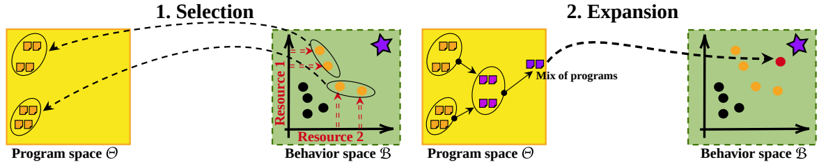
Figure – Schematic view of the goal achievement strategy for a combination of two resources. For each resource r \in c the combination, one selects the k closest outcomes from the database \mathcal{H} (yellow), and one expands by producing a candidate parameter (purple), and this involves first mixing the selected pairs of programs for resource 1 and resource 2 separately, then mixing the results.
