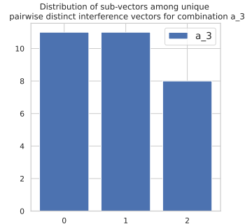
Figure – Among the set of pairwise distinct vectors for combination a_3 \in \mathcal{S} , distribution of the subvectors featuring a selection of values.
