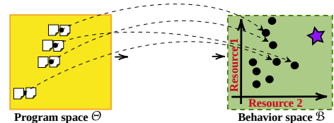
Figure – Schematic view of the goal sampling process. The purple star represents the goal in the behavior space. The axis indicate the agent tries to reach an experiment outcome with at least one interference for each required resource.
