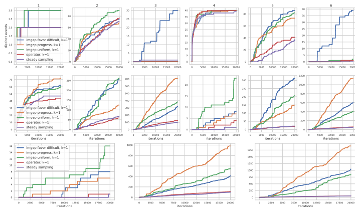
Figure – Evolution over the exploration of the number of distinct events for the different combinations of interference types. This results from the same example runs than figure 5
