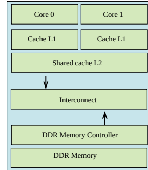
Figure – Simulated dual-core architecture used in this work.
