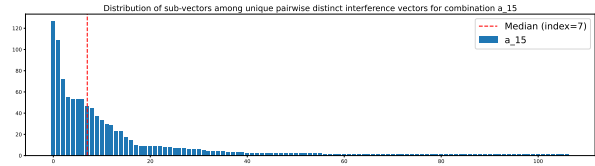
Figure – Among the set of pairwise distinct vectors for combination a_{15} \in \mathcal{S} , distribution of the subvectors featuring a selection of values. We see that median is 7, meaning that only 7 distinct vectors are responsible for 50 pourcents of the interference.
