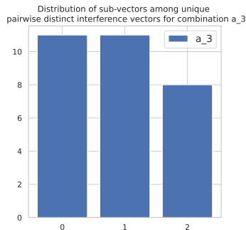
Figure – Among the set of pairwise distinct vectors for combination a_3 \in \mathcal{S} , distribution of the subvectors featuring a selection of values.
