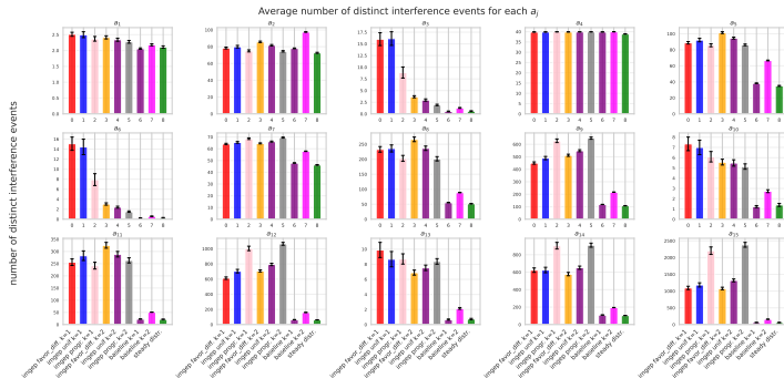
Figure – Number of distinct events for each resource combinations. This results from an example run of N = 2 \cdot 10^4 IMGEF iterations with k = 1, 2, 3 and a warming set of N_{init} = 1000 iterations of random program synthesis, and 3 random mutations from the mutation operator.
