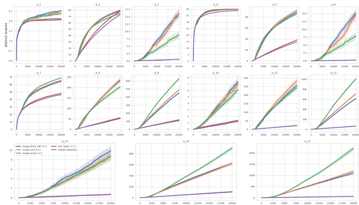
Figure – Evolution over the exploration of the number of distinct events for the different combinations of interference types. This results from the same example runs than presented on figure 5
