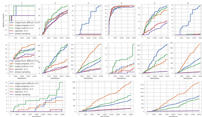
Figure – Evolution over the exploration of the number of distinct events for the different combinations of interference types. This results from the same example runs than figure 4
