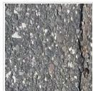
CRACK500
