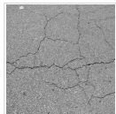
cracktree200
